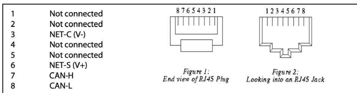
Victron VE.Can pinout
