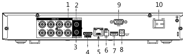
DH-XVR5108H-I
